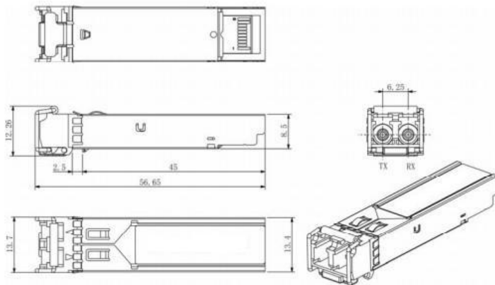
Mechanical Drawing
