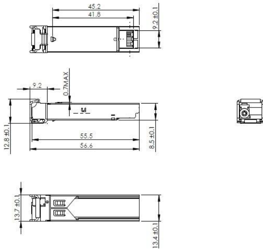
Mechanical Drawing
