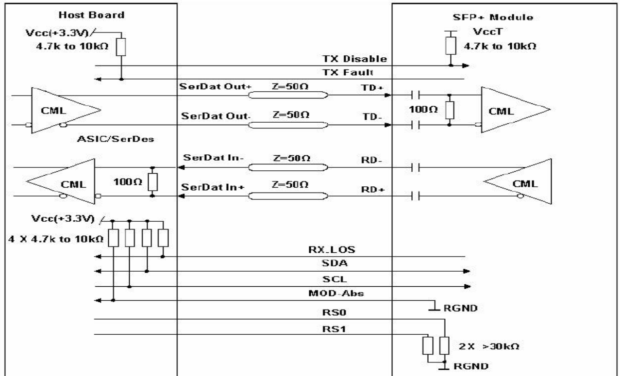
Recommended High-speed Interface Circuit
