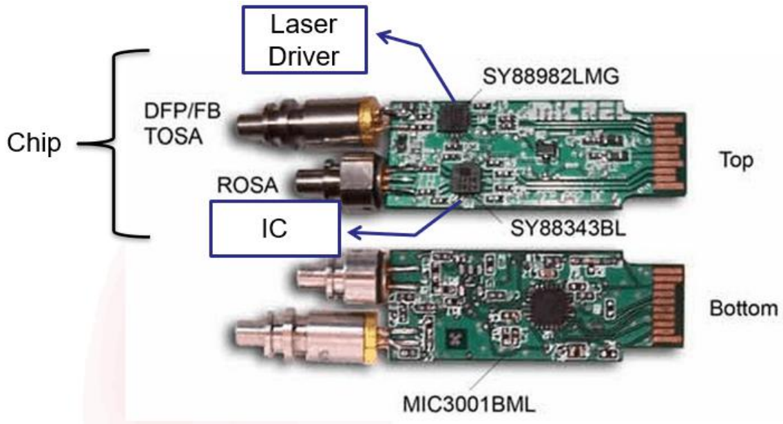
Composition of the general model with main components
