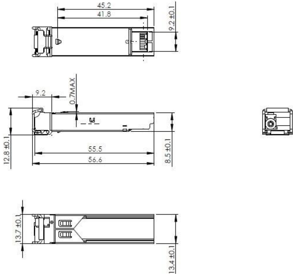
Mechanical Drawing
