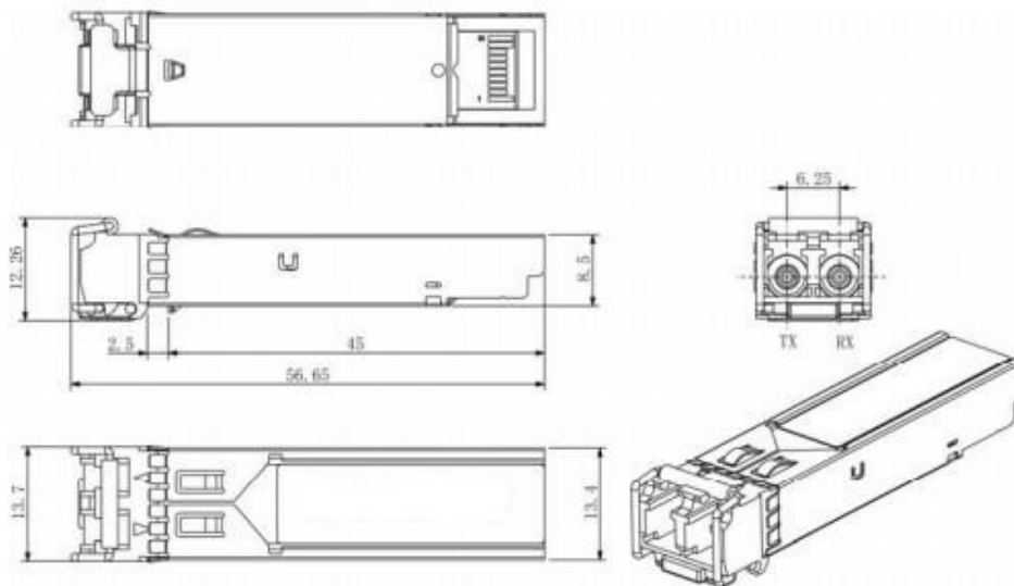
Mechanical Drawing
