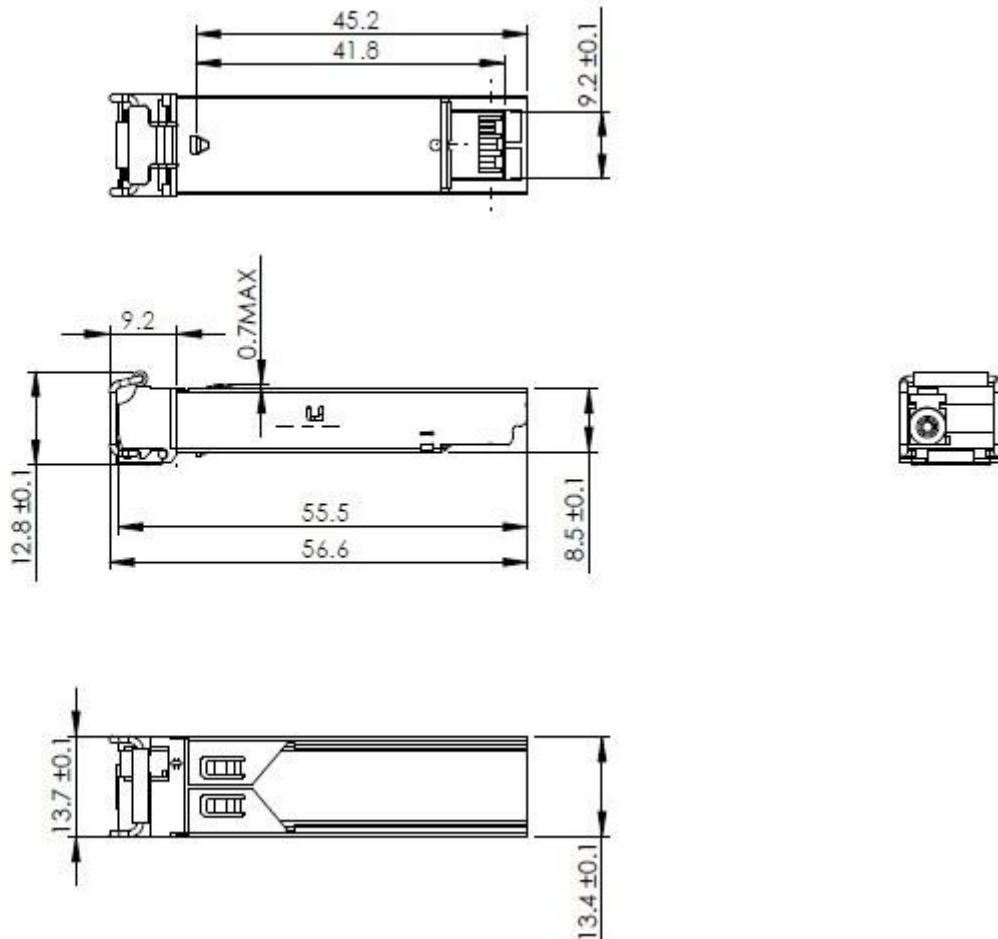
Mechanical Drawing
